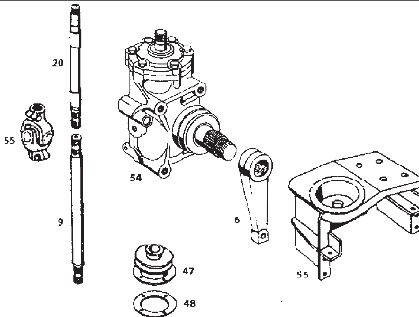
FITMENT OF ZP POWER STEERING
