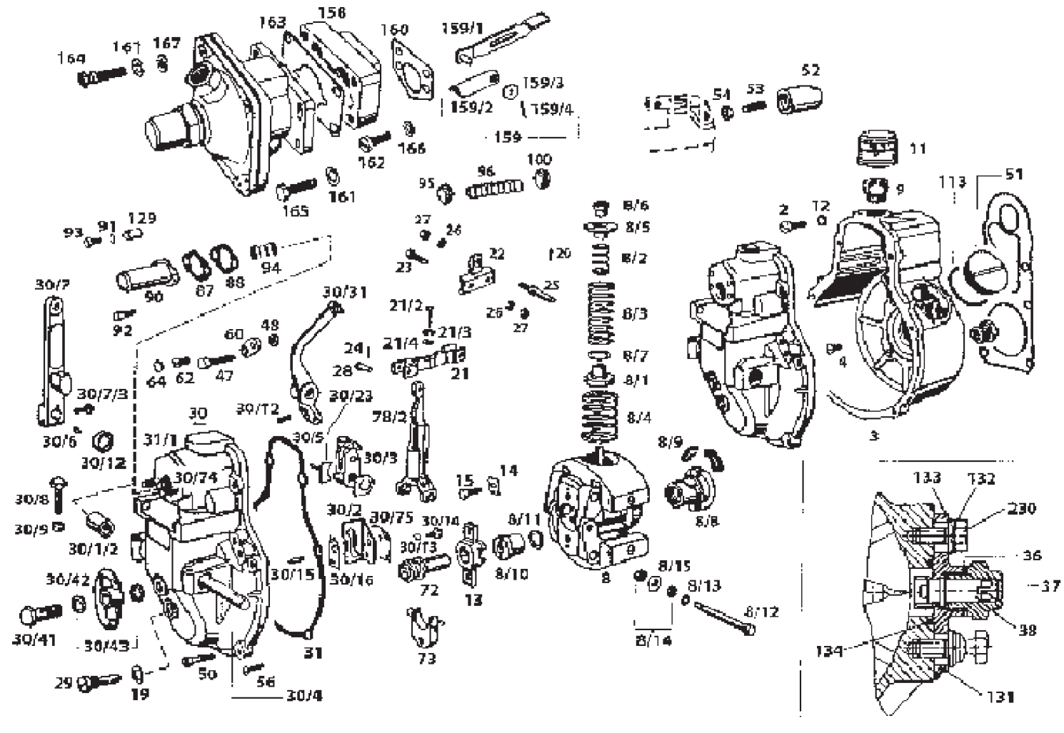
GOVERNOR (MICO)
