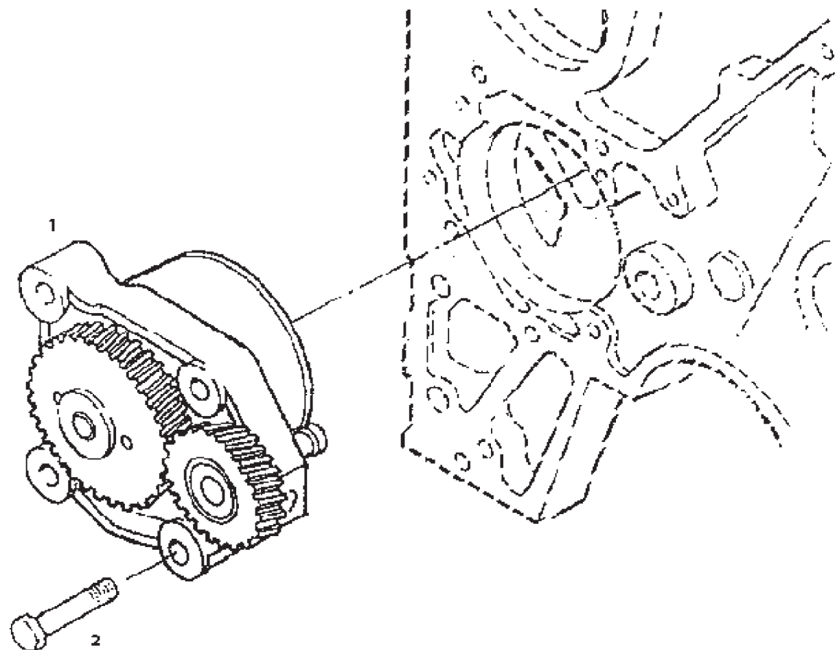
LUBRICATING OIL PUMP
