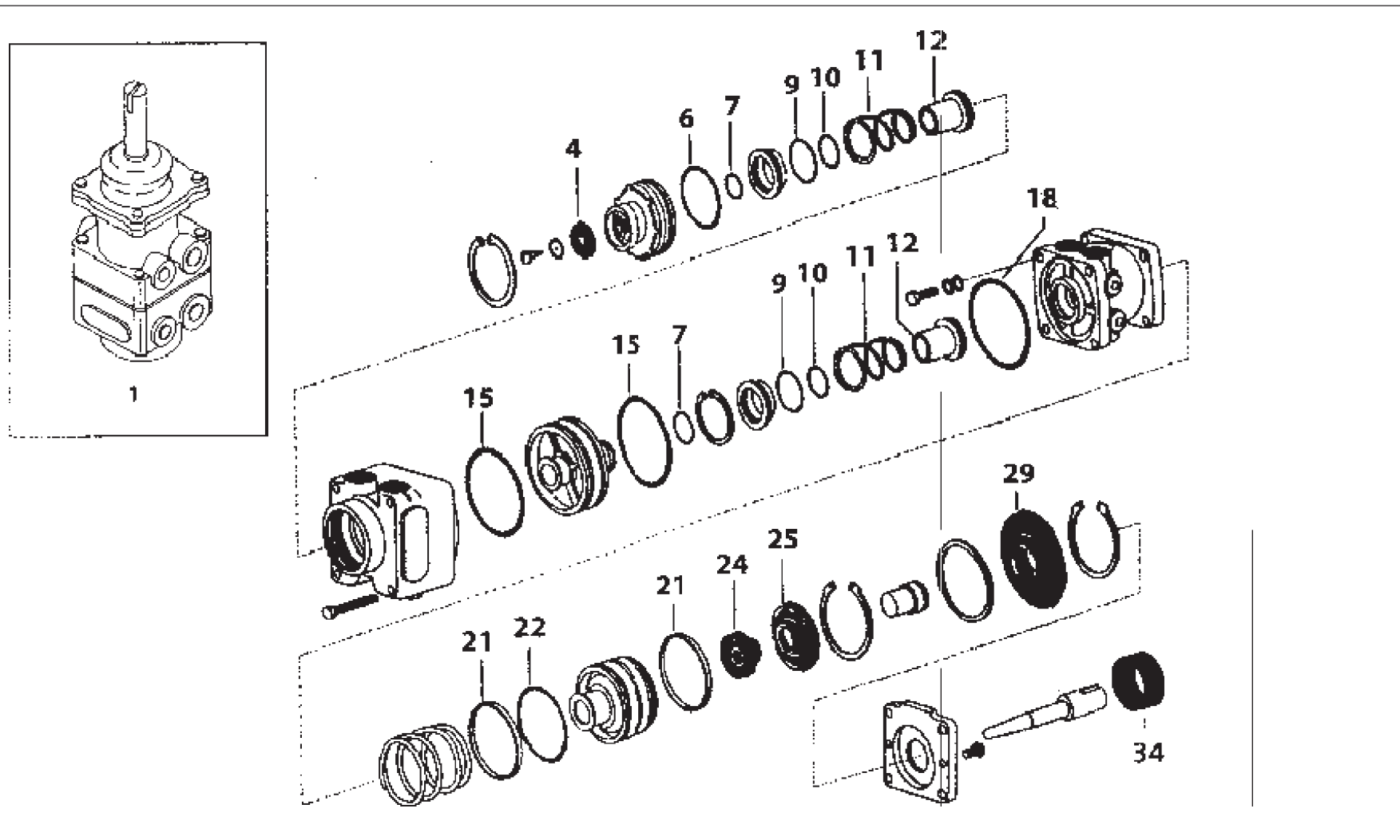
DUAL BRAKE VALVE
