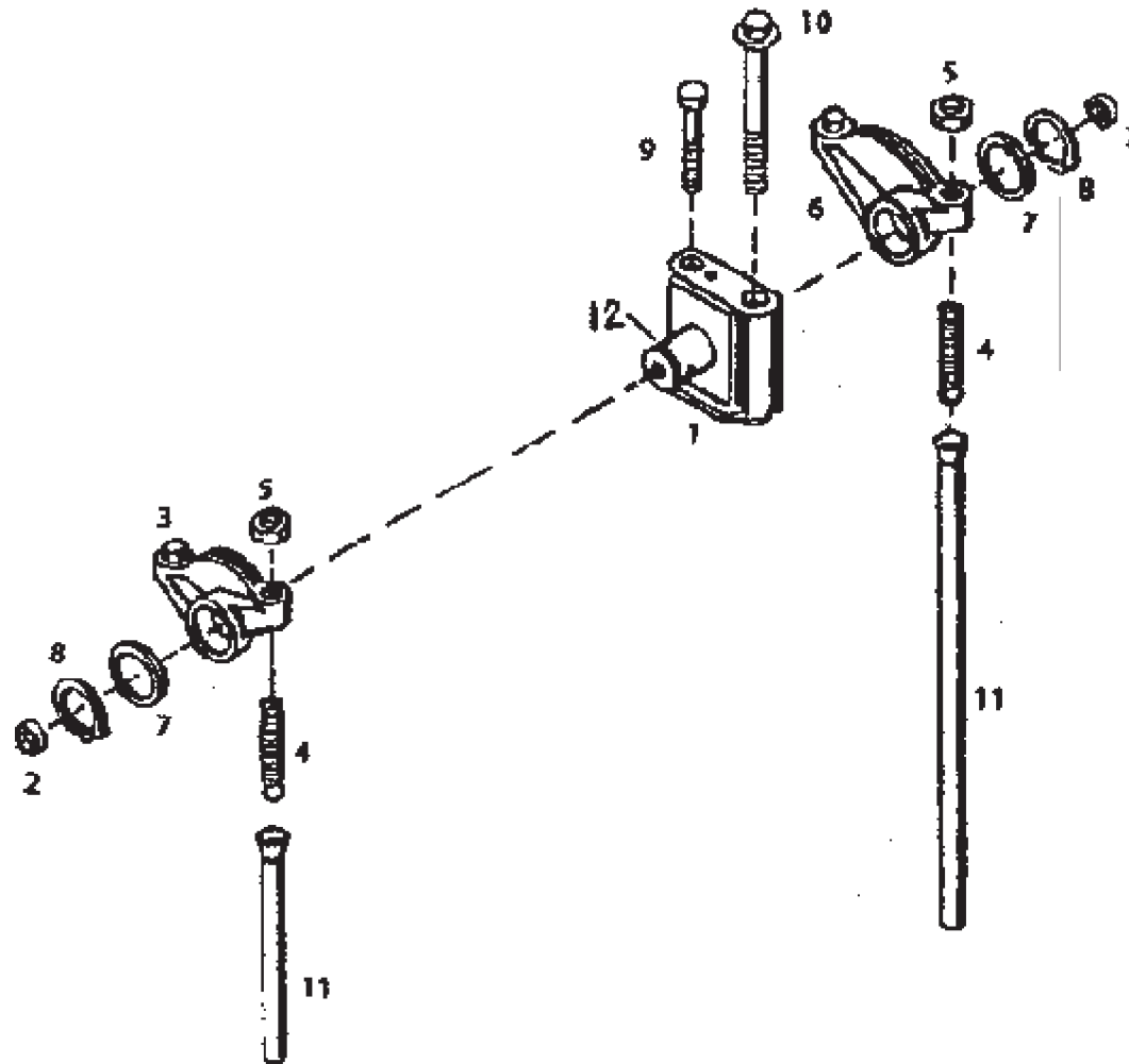
ROCKER LEVER
