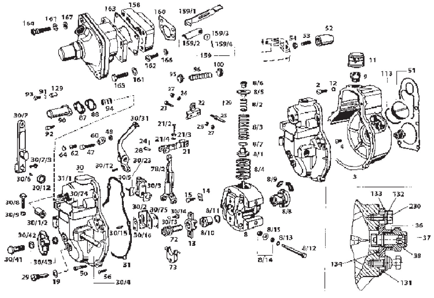
GOVERNOR (MICO)
