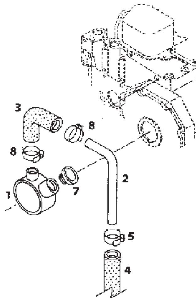
BREATHER CRANKCASE
