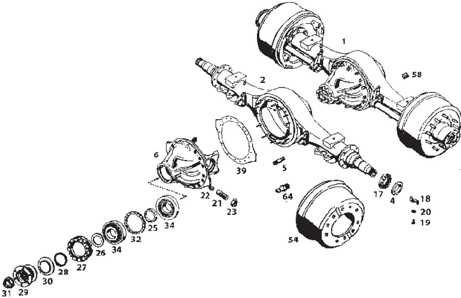
REAR AXLE RA 109
