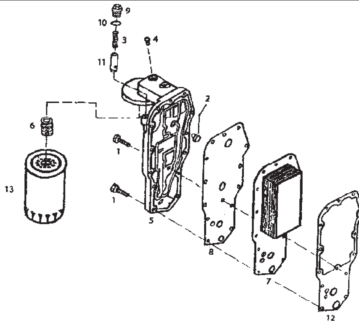
LUBRICATING OIL COOLER/OIL FILTER
