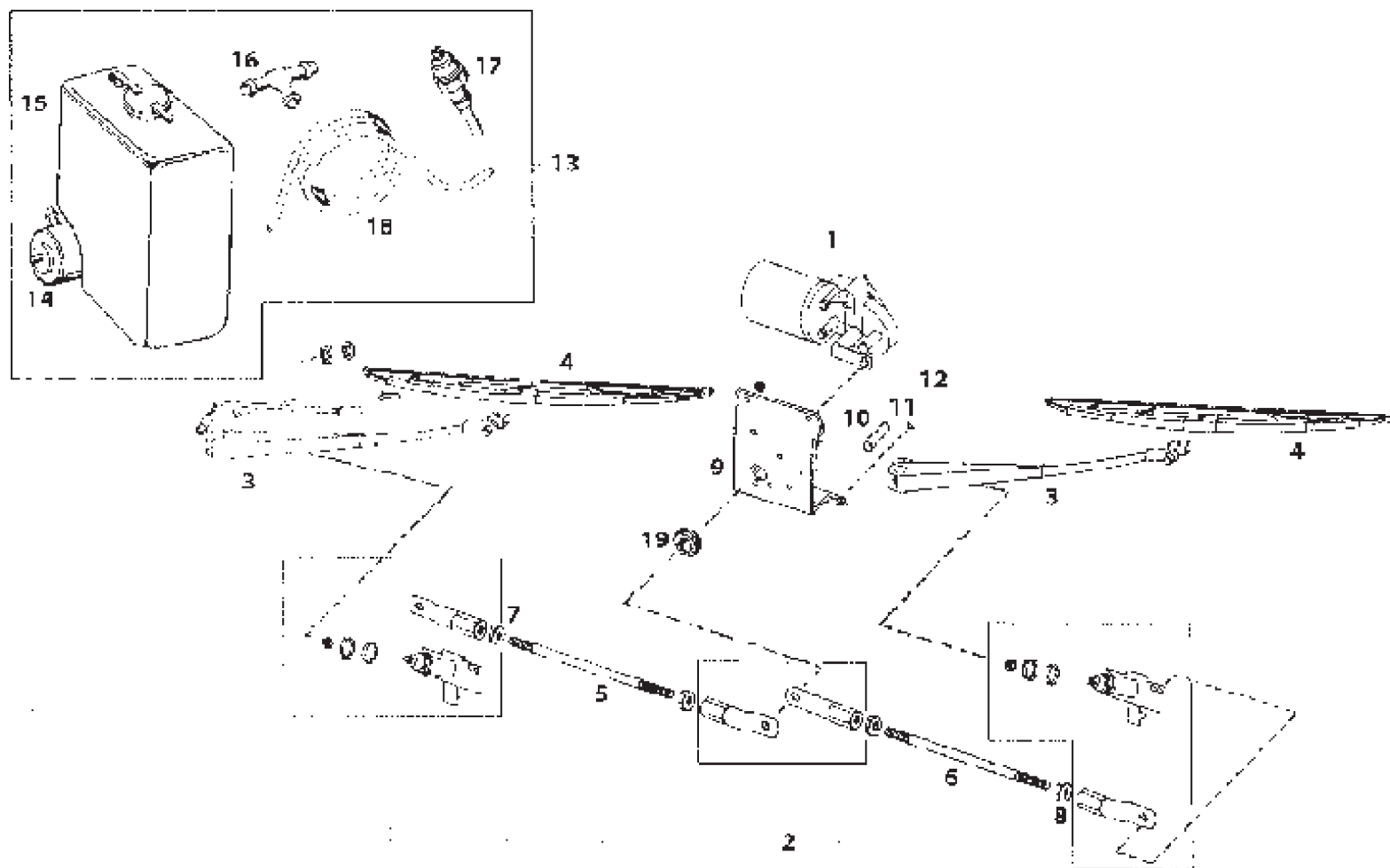
WIPER, WINDSHIELD WASHER ARRANGMENT
