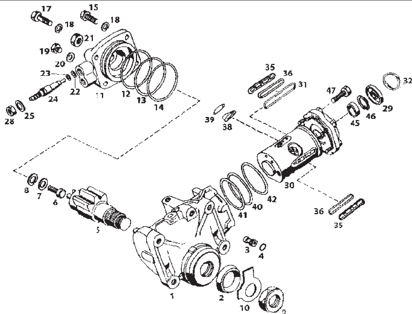
STEERING GEAR BOX (ZF INDIA)
