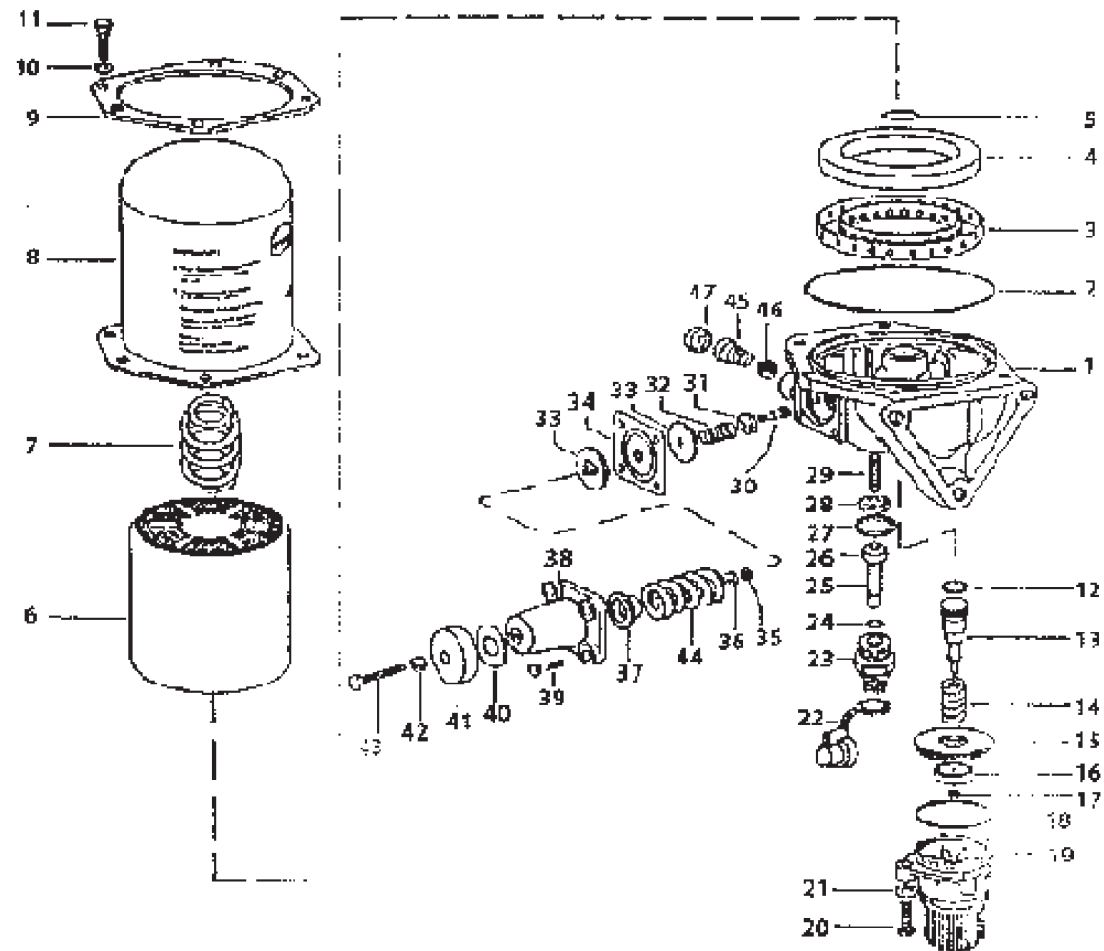
AIR DRYER
