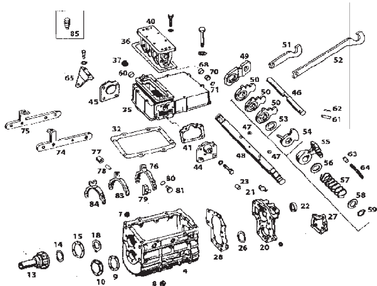
GEAR BOX ASSY.GBS 50
