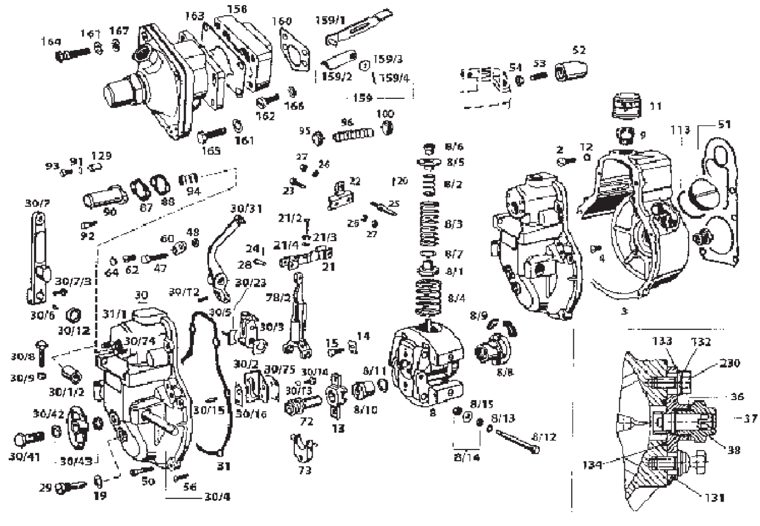
GOVERNOR (MICO)
