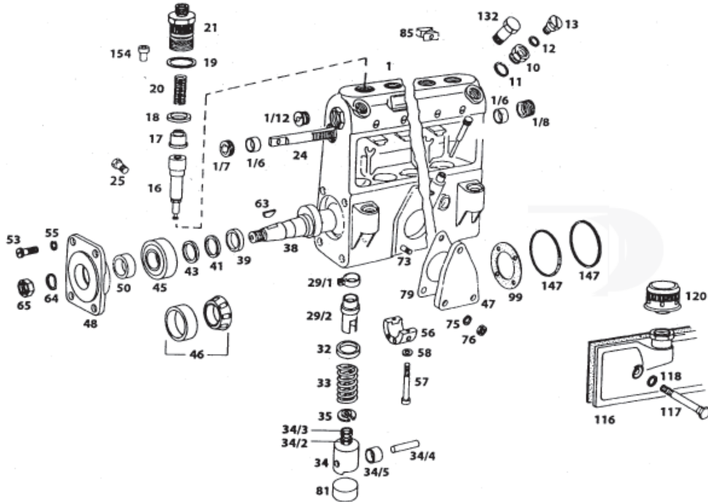
FUEL INJECTION PUMP (MICO)
