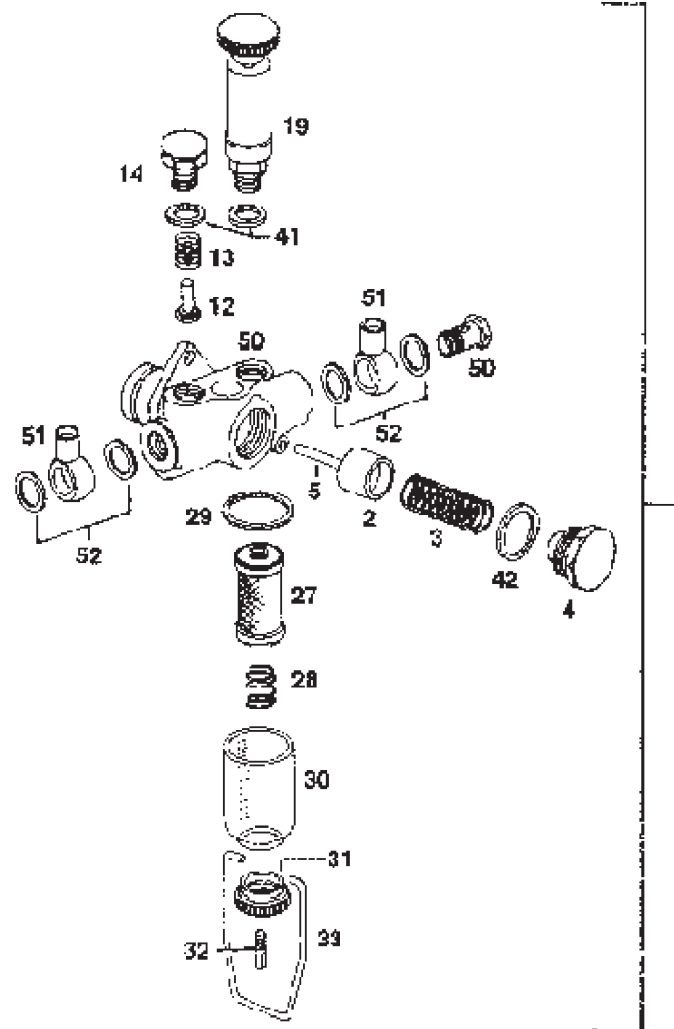
FUEL FEED PUMP
