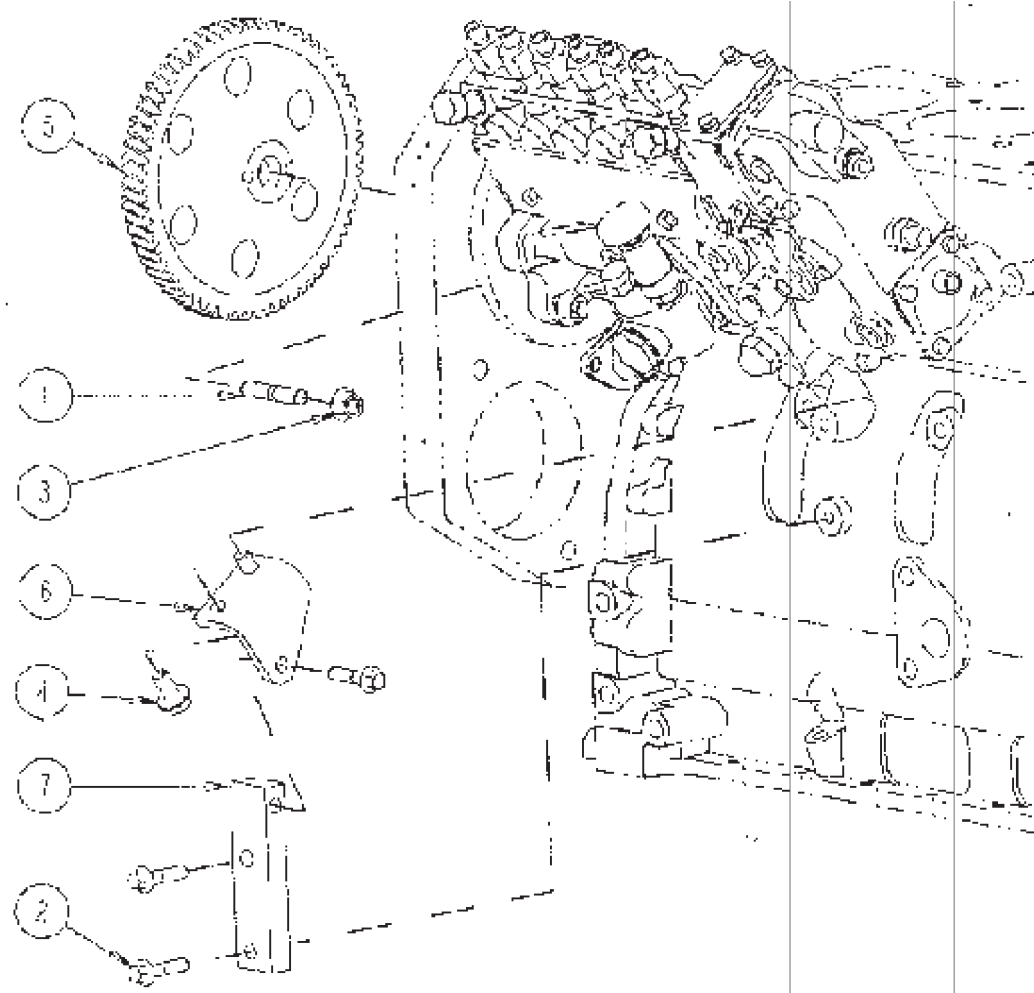
COUPLING FUEL PUMP
