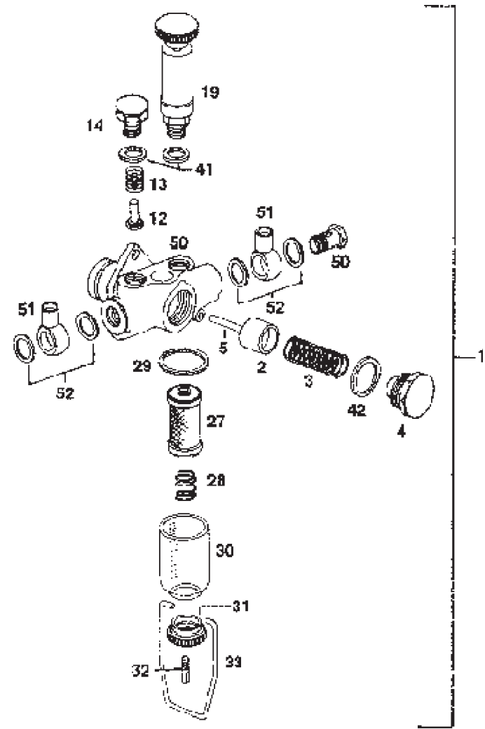
FUEL FEED PUMP
