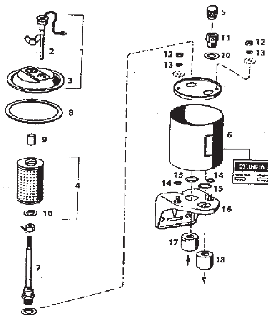
HYDRAULIC TANK FOR POWER STEERING (ZF INDIA)
