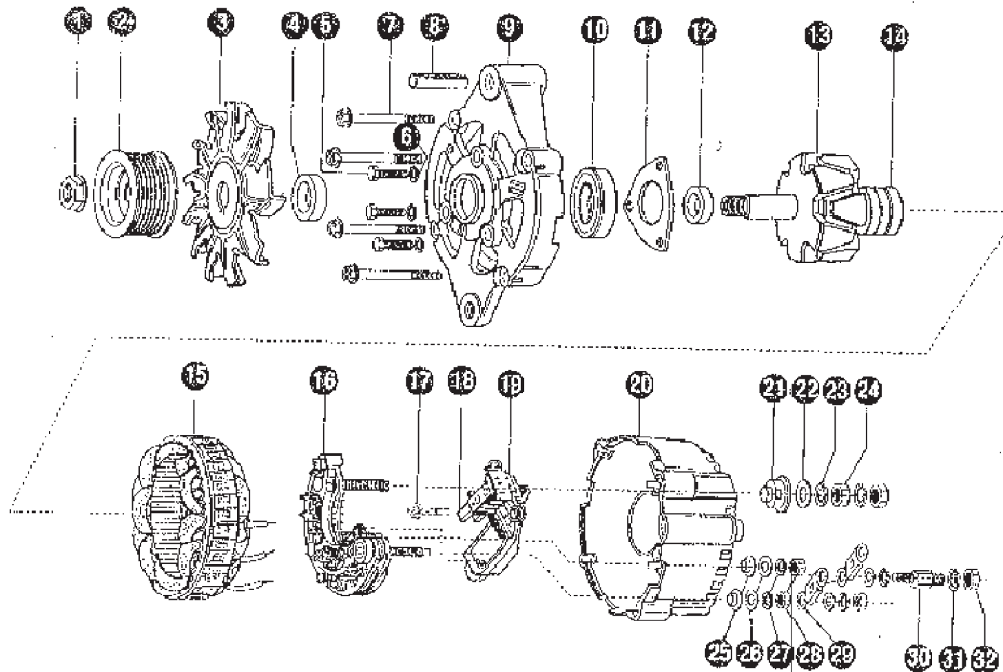
COMPONENT DETAILS OF ALTERNATOR
