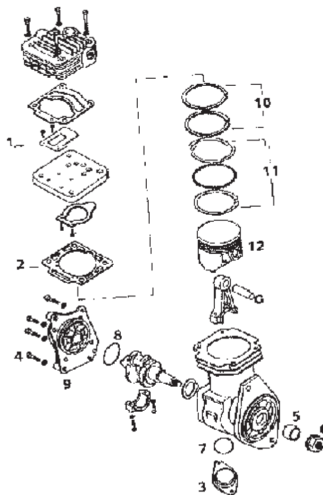
REPAIR KIT FOR AIR COMPRESSOR
