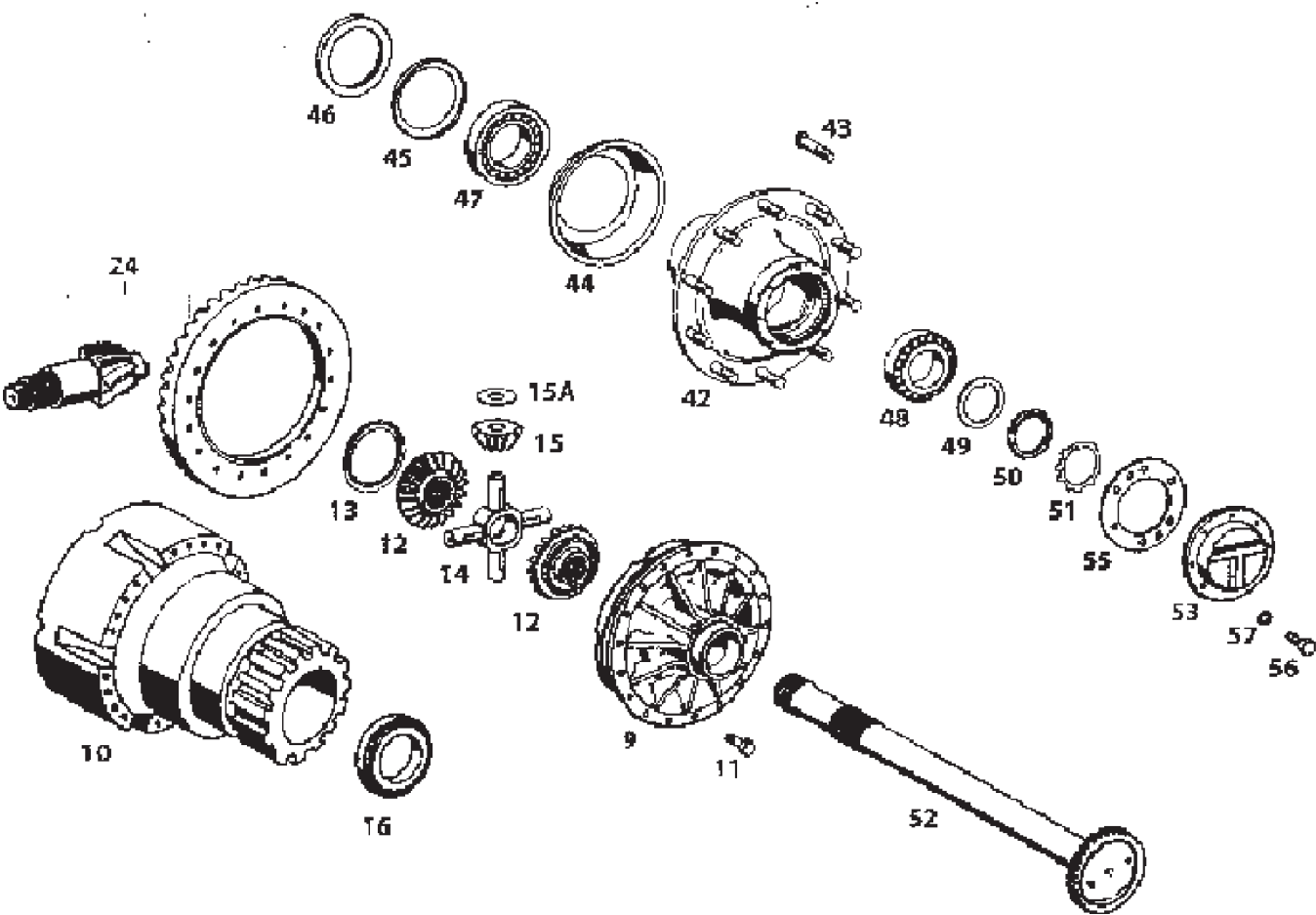
REAR AXLE RA 109
